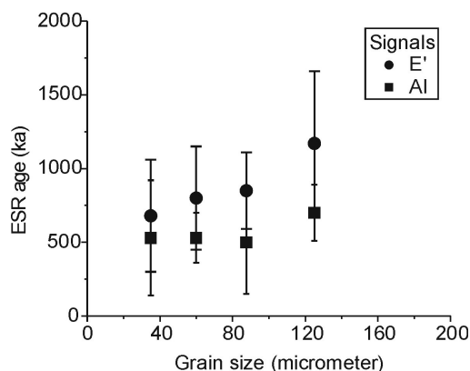
Fig. 16: ESR age plot for fault gouge from the Wangsan Fault (Southern Korea) according to the grain size and the ESR centre used. Note the systematically higher ages for the E' -centre. Replotted after LEE & YANG (2003).
